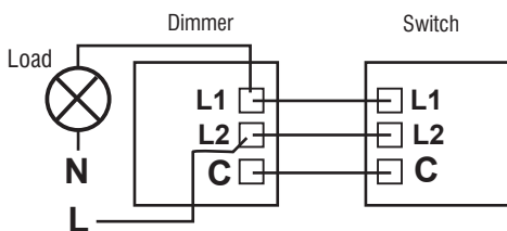
Diagram 2: Using a 2 way dimmer switch Dimmer must replace only one of the 2 way switches
