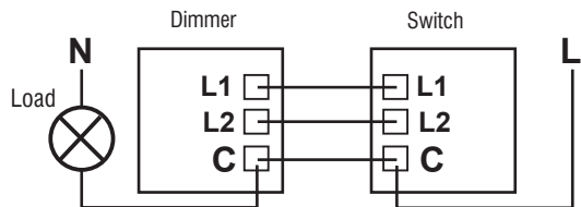
Diagram 3: Using a 2 way dimmer switch Dimmer must replace only one of the 2 way switches
